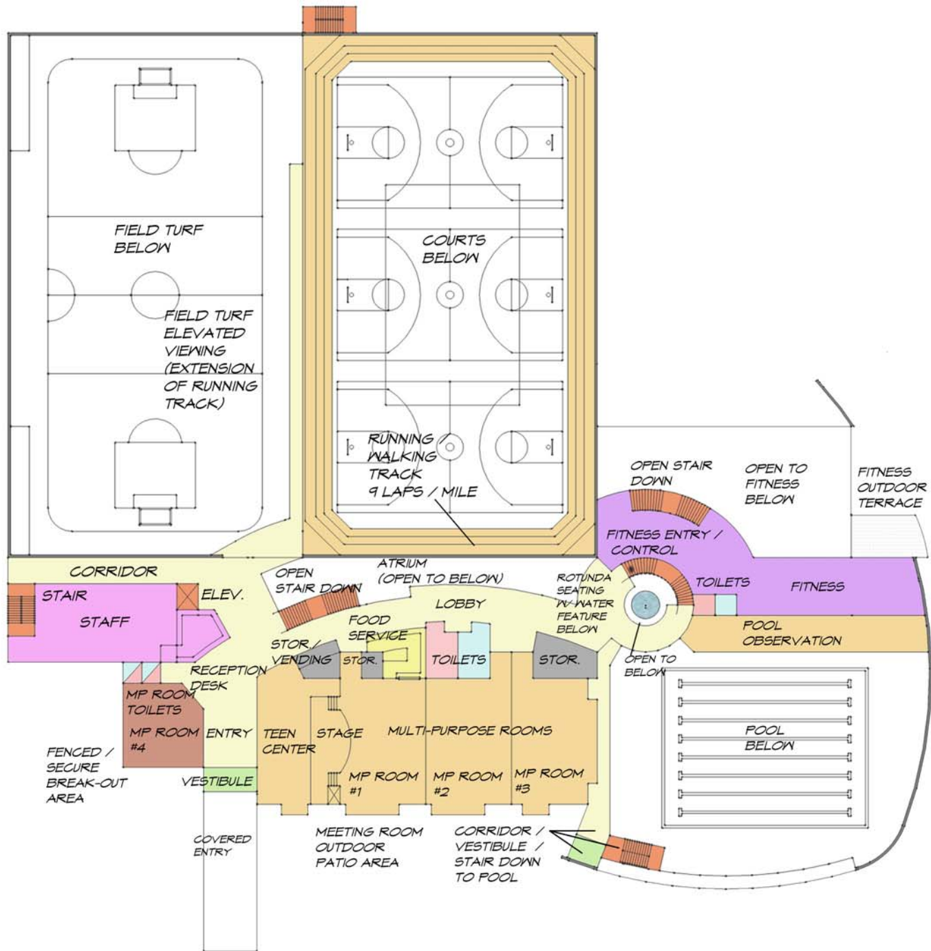
Conceptual Main Level Floor Plan Scale 1"= 50'-0" on 8.5 x 11 Sheet
