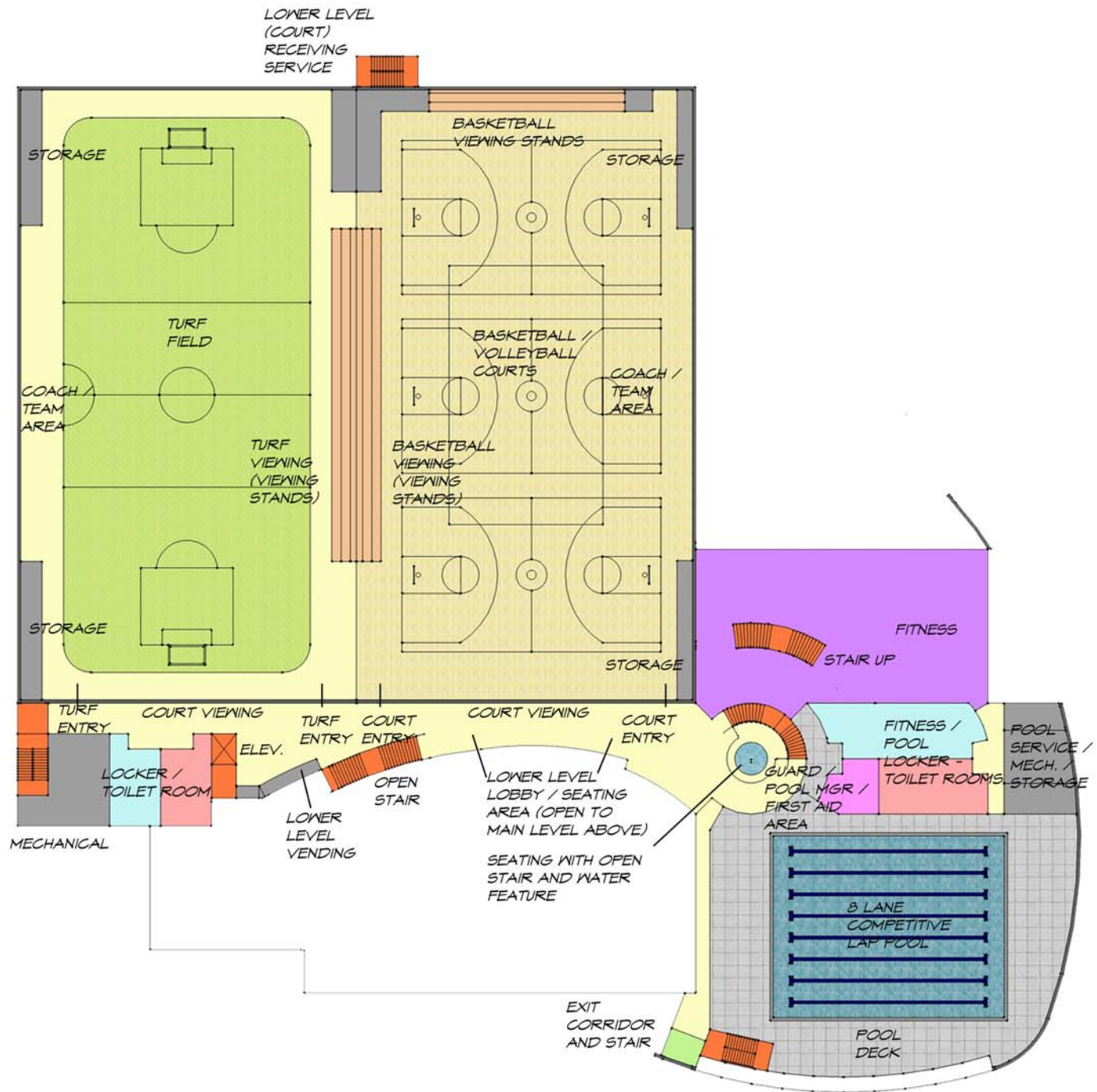
Conceptual Lower Level Floor Plan Scale 1" = 50'-0" on 8.5 x 11 Sheet
